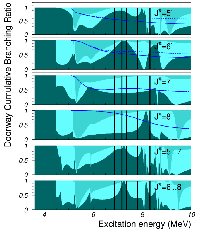
FIG. 5. A cumulative plot of calculated neutron branching ratios of J^\pi = 5^-, 6^-, 7^-, 8^- ^{134}\text{Sn} states as a function of excitation energy with the doorway interpretation using neutron L = 6 emission from 0i_{13/2} . The predictions of the Hauser-Feshbach model for a given spin are shown for comparison: solid blue line represents feeding to 7/2^- state and dashed blue line to 3/2^- . The last two plots show average cumulative branching ratios expected in the Gamow-Teller decay for the ^{134}\text{In} ground state spins of J^\pi = 6^- and J^\pi = 7^- , respectively.
